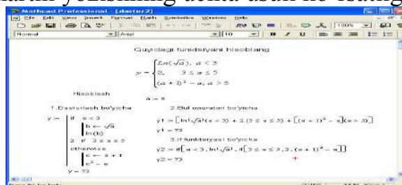
2-rasm. Shartli funktsiyani uch usulda hisoblash.
