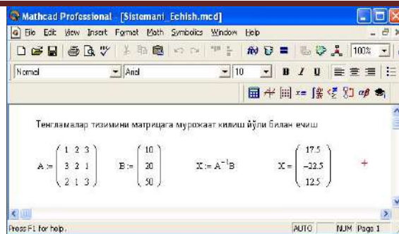
3-rasm. Tenglamalar tizimini matritsa usulida yechish.
