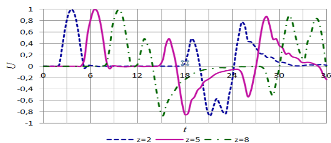
2-chizma. Elastik sterjenda ko'chishning vaqt davomida o'zgarishi ( t_1=3 , \Omega=0 )
