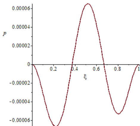
W_0^{(0)*}(x, t)
